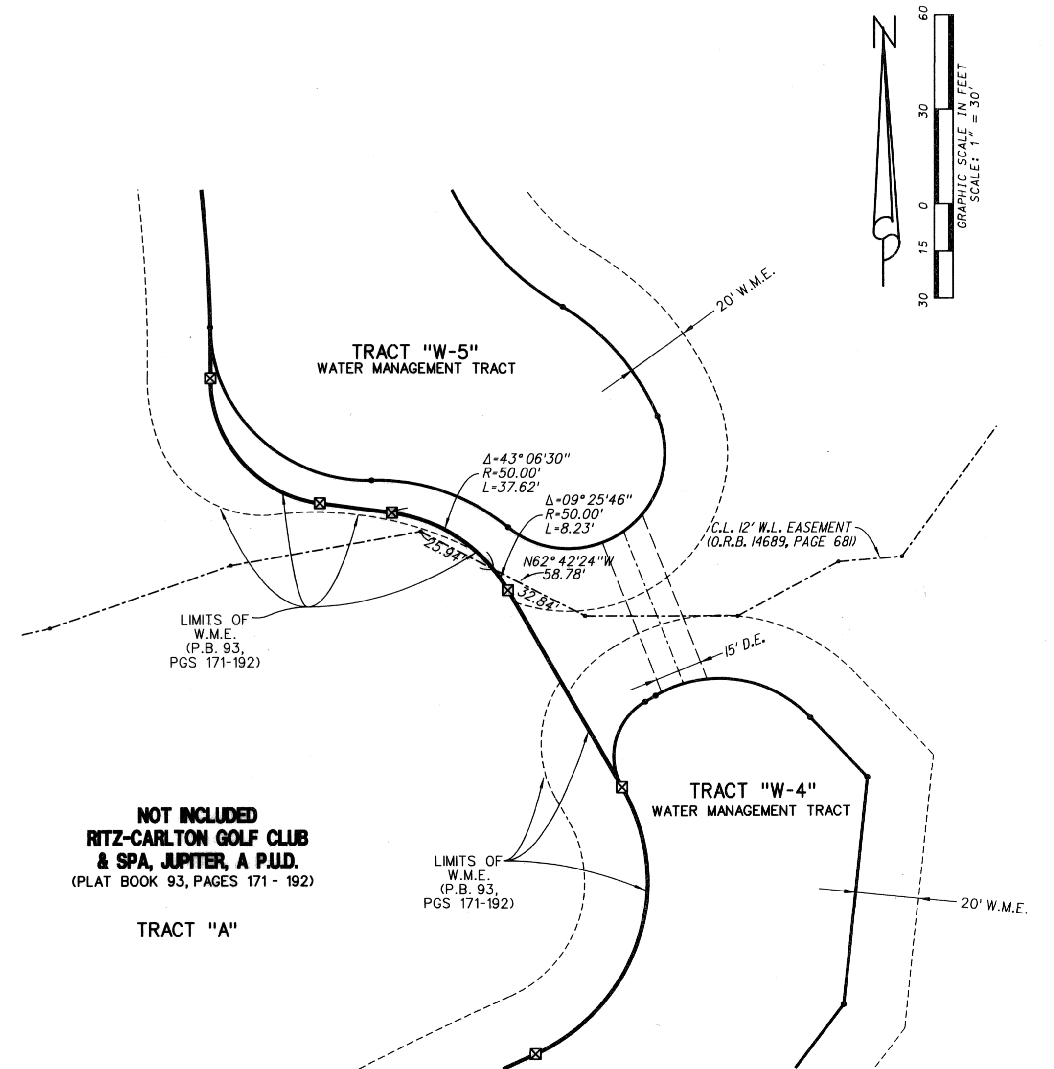
DETAIL "B"
