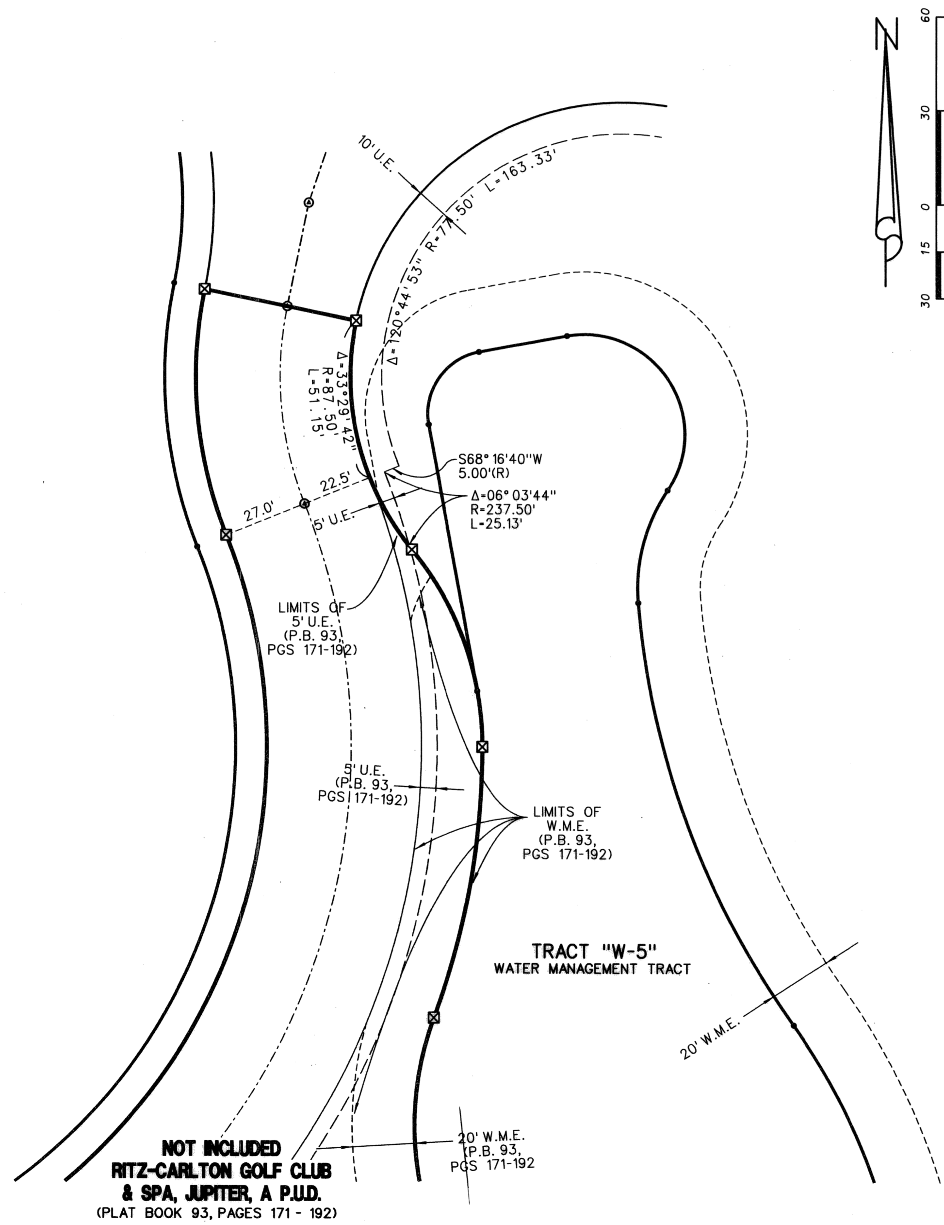
DETAIL "A"
